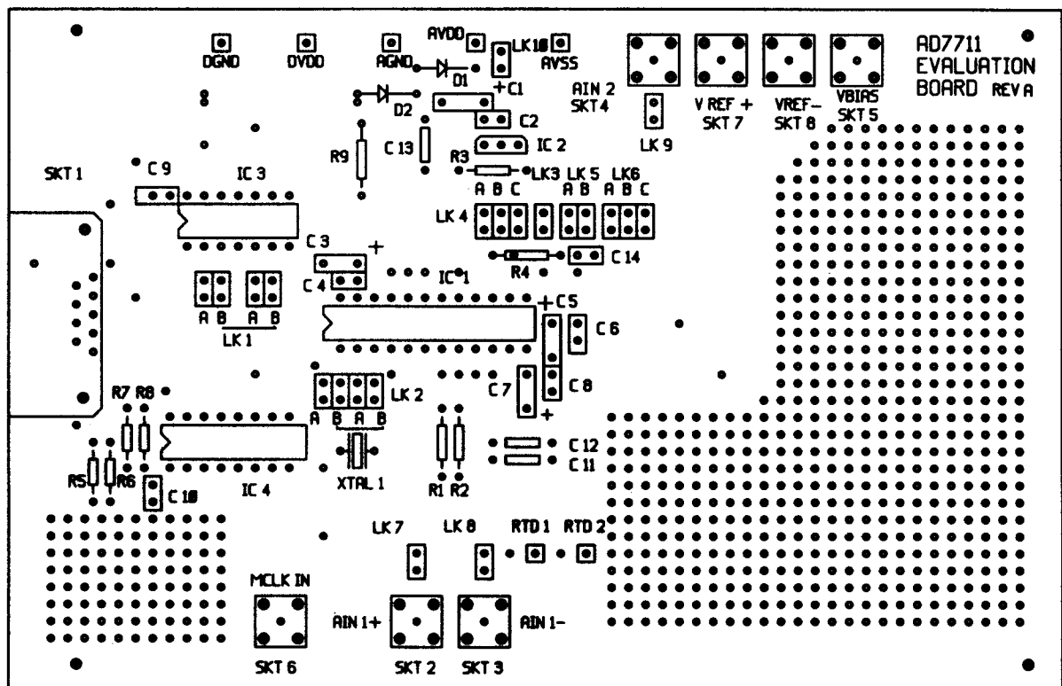
Figure 4. AD7711 Evaluation Board Silkscreen
